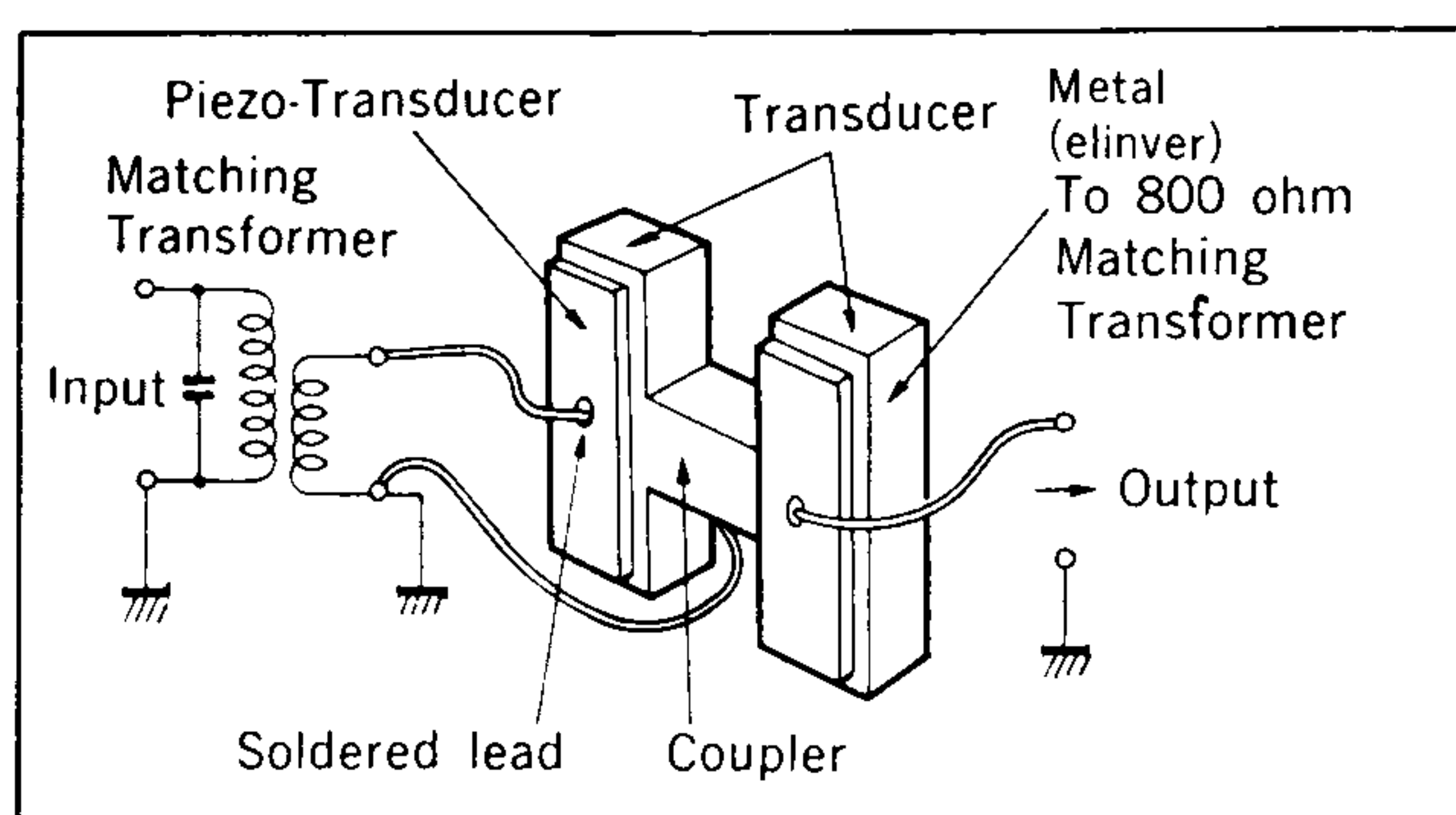
Figure 2 — Mechanical Filter
