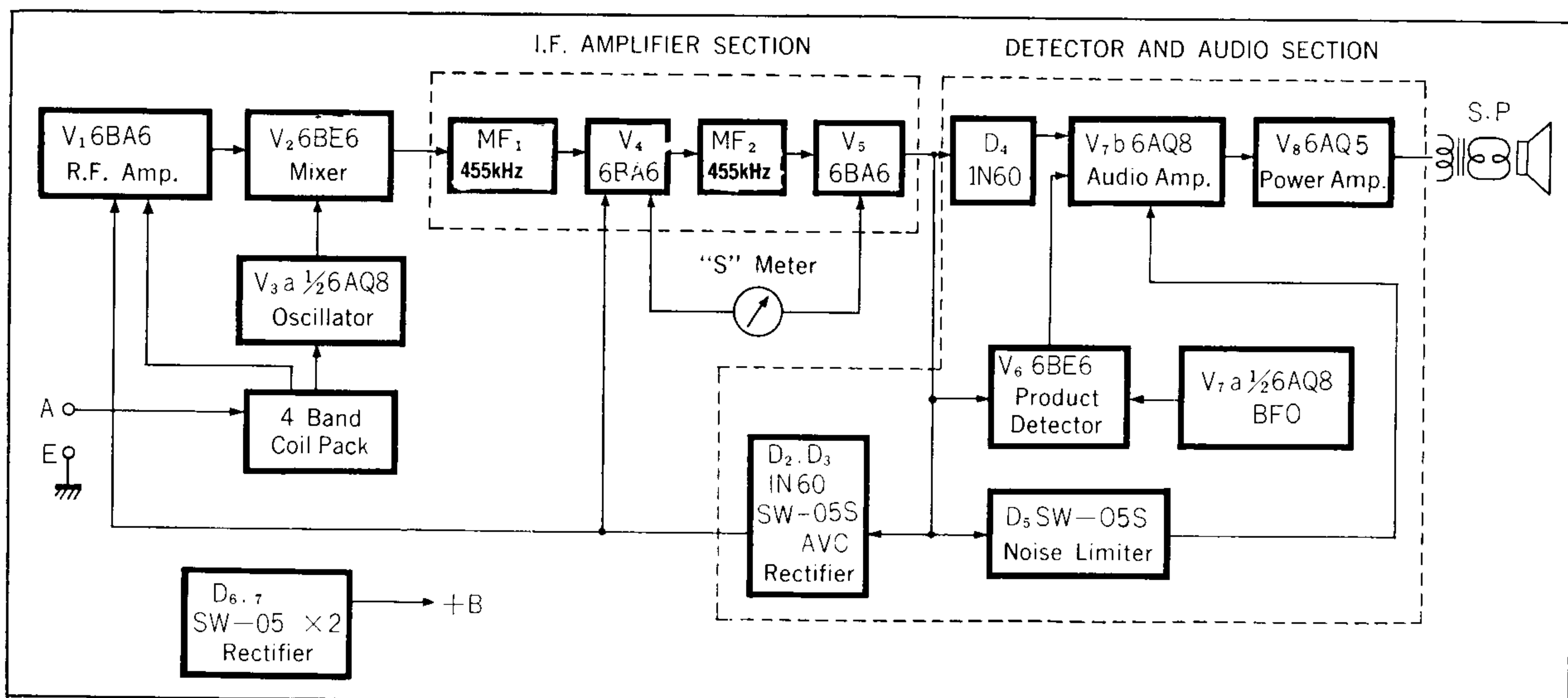
Figure 1 — Block Diagram
